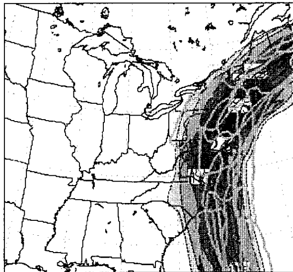
Figure 5. Probability of 2 inches (50 mm) of rain in 36 hours and spread from the SREF initialized 09Z 7 October 2005 and Valid 12Z 8 October 2005 through 00Z 10 October 2005.
