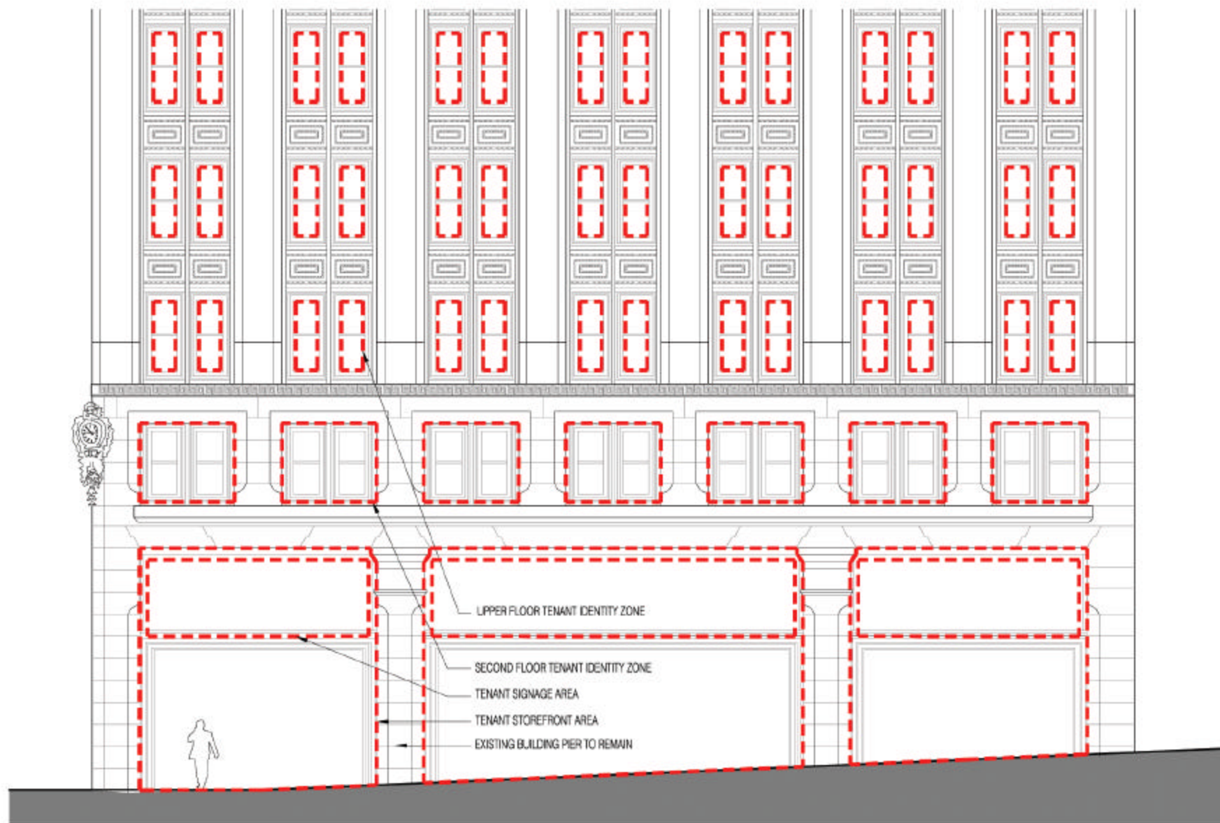
DRAFT TENANT IDENTITY ZONES EXHIBIT 2 Jones, McDuffee, and Stratton Company Building, 1905 April 28, 2006 Scale: 3/32"=1'-0"
