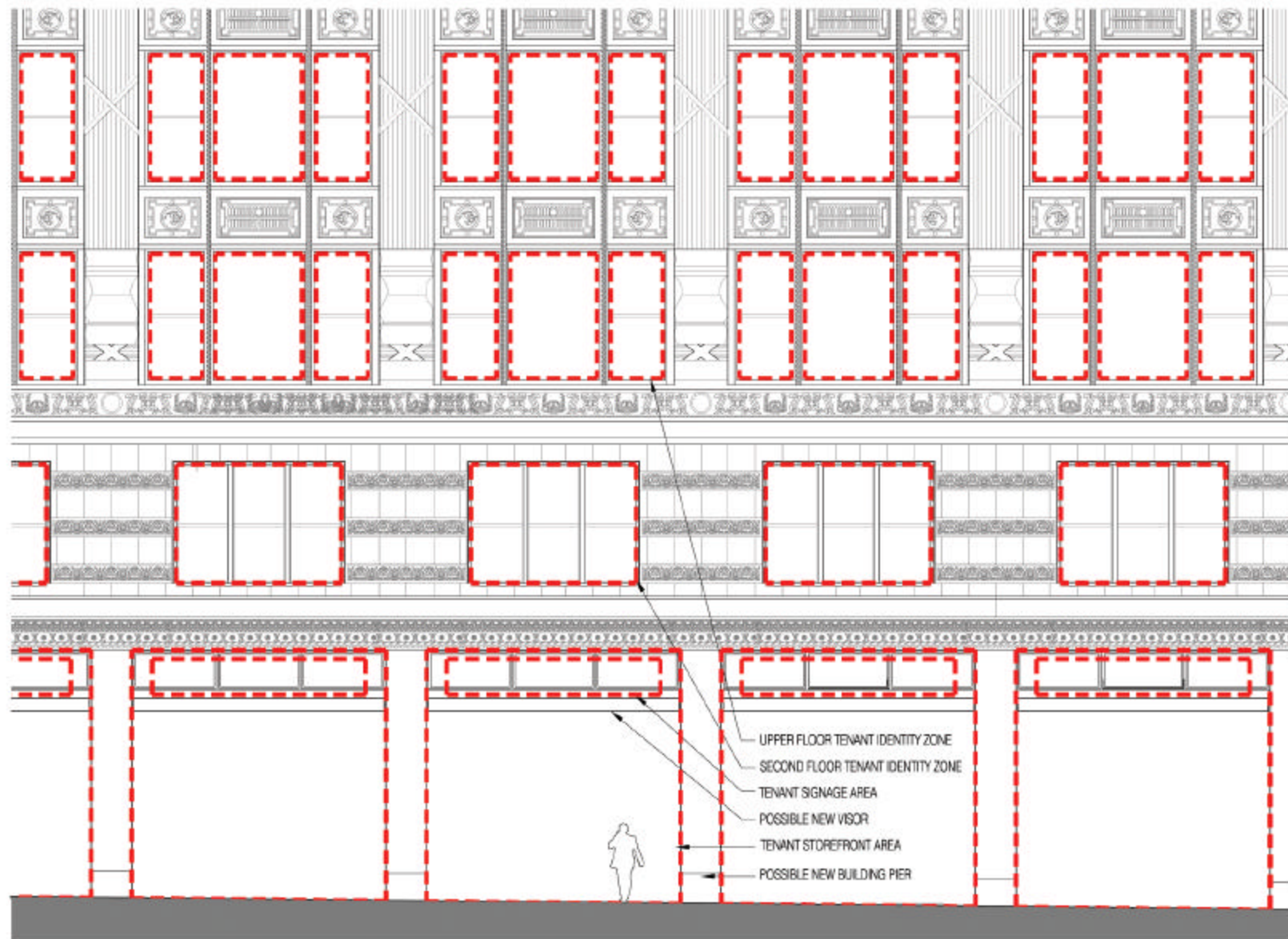
DRAFT TENANT IDENTITY ZONES EXHIBIT 1 1912 PURPOSE BUILT FILENES BUILDING April 28, 2006 Scale: 3/32"=1'-0"
